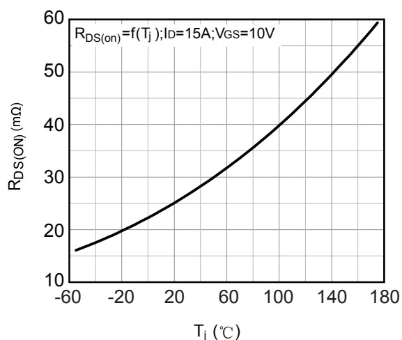
Typ. Drain-Source on-state resistance
